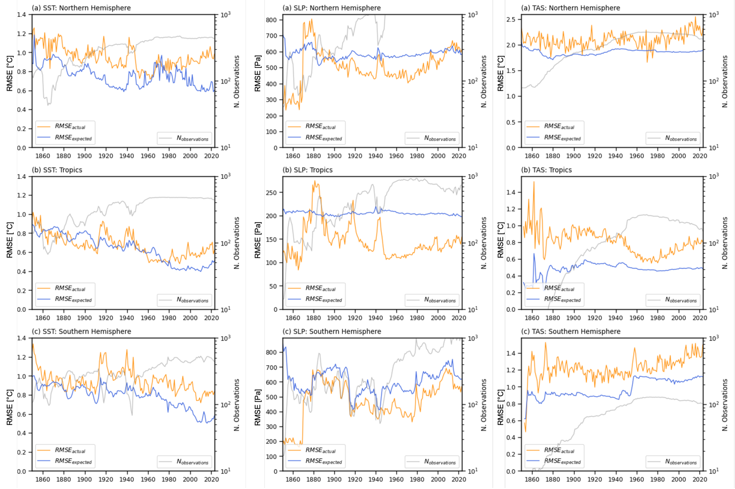
Figure S6. Desroziers validation statistics. (Left column) Actual versus expected RMSE averaged for sea-surface temperature over (a) the Northern Hemisphere from 20^{\circ} – 90^{\circ} N, (b) the Tropics from 20^{\circ} S– 20^{\circ} N, and (c) the Southern Hemisphere from 20^{\circ} – 90^{\circ} S. The annual-mean number of observations assimilated per month is shown in gray (right vertical axis). Note that the vertical axes differ between subplots. (Middle column) Same as left column for sea-level pressure. (Right column) Same as left column for near-surface air temperature. All time series show annual means.
