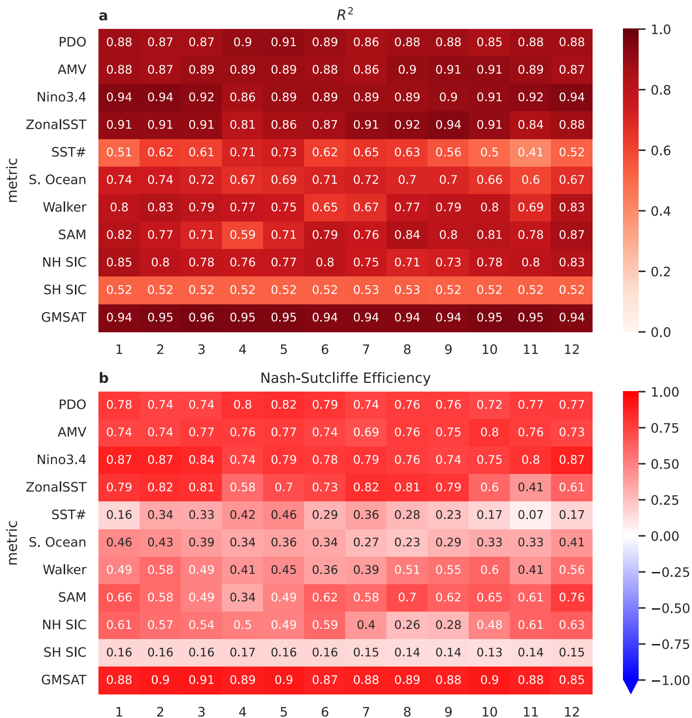
Figure S5. Validation by pseudo-reconstruction of MPI-ESM1-2-HR: squared Pearson's correlation and Nash-Sutcliffe efficiency by month. Metrics on the vertical axis correspond to those in Figure 2 but the calculations are based on the monthly resolved data without any low-pass filtering. The horizontal axis represents months January–December. Calculation is over the full pseudo-reconstruction period (1850–2014).
