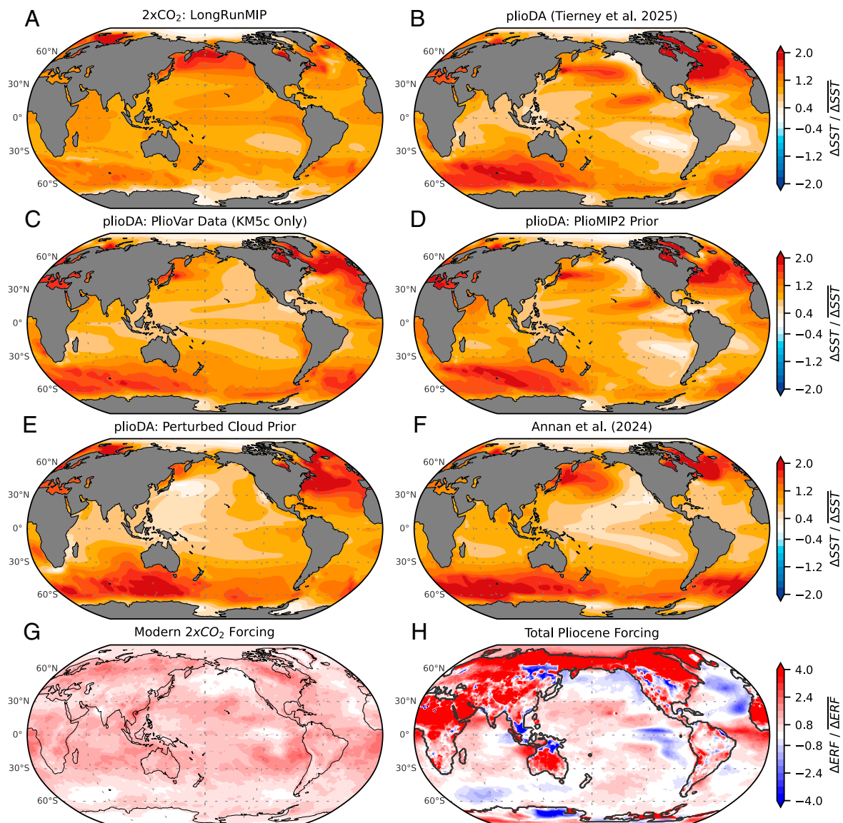
Fig. 1. Patterns of sea-surface temperature (SST) anomalies and effective radiative forcing (ERF). (A) Multimodel mean of modern SST response to 2\times\text{CO}_2 in quasi-equilibrium simulations from LongRunMIP (32). (B–F) Data-assimilation reconstructions from: (B) plioDA best estimate (12); alternative plioDA using (C) only the PlioVar proxy data representing the KM5c interglacial, (D) only the PlioMIP2 prior, or (E) only the perturbed-cloud prior; and (F) best estimate from ref. 13. ERF from (G) modern 2\times\text{CO}_2 and (H) Pliocene total forcing, including greenhouse gases, reduced Greenland and Antarctic ice sheets, sea level, topography, and vegetation (24). All panels show annual-mean anomalies, and local values are divided by global means. Pliocene SSTs are infilled to modern coastlines.
